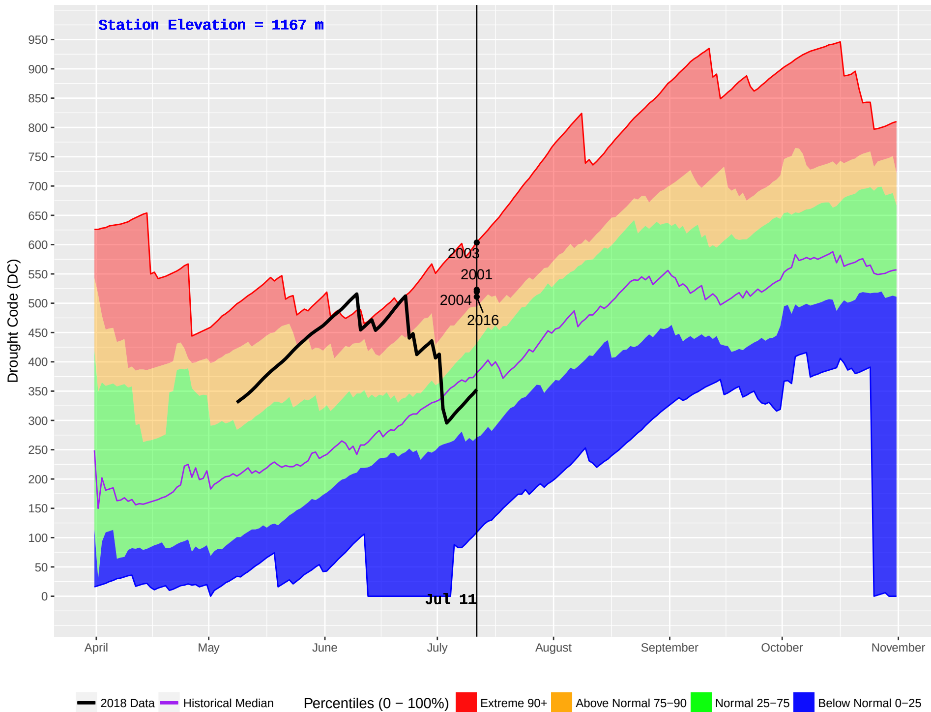
LEIGHTON LAKE (307) : Historical (1982–2016) and Current (2018) Noon Drought Code (DC)
