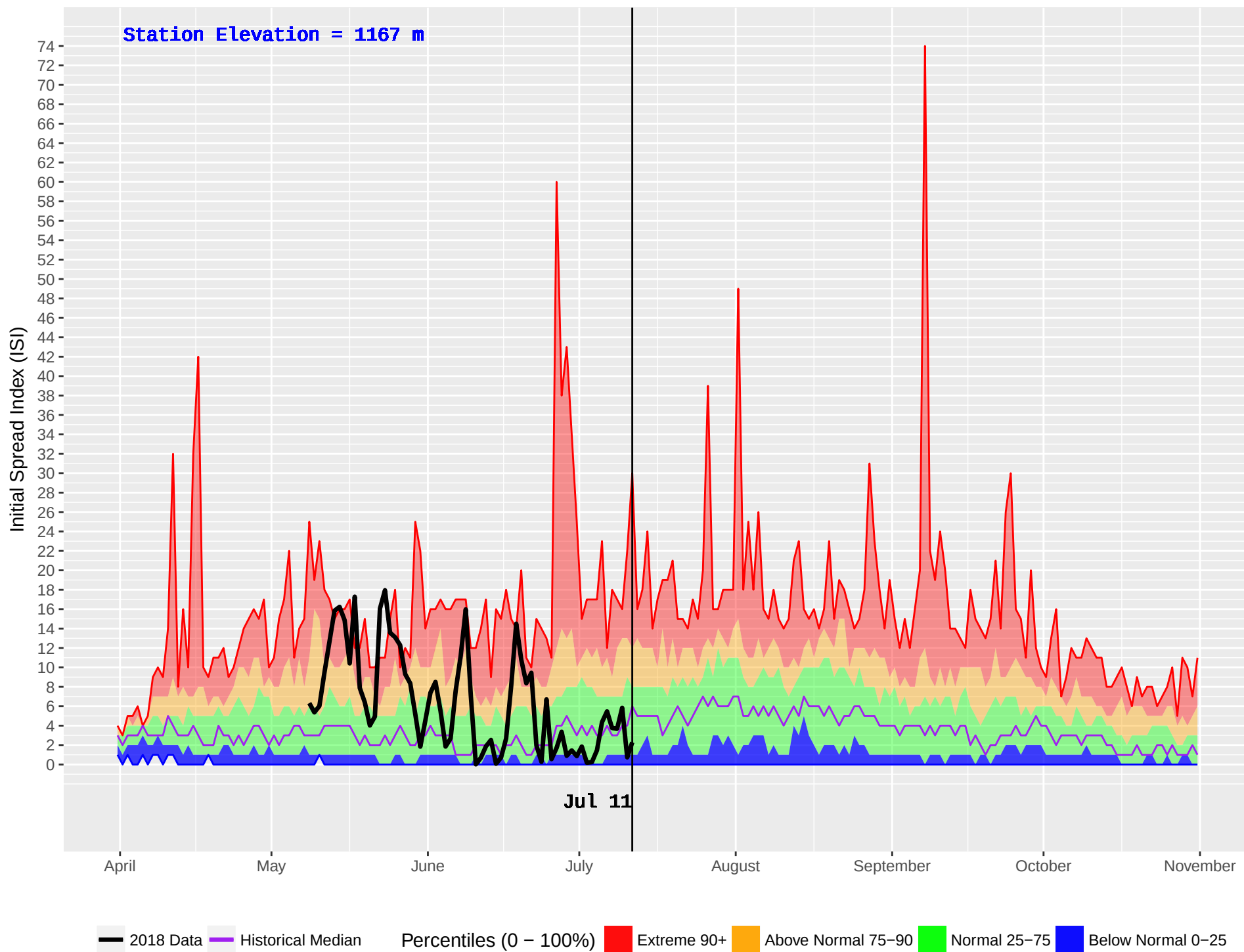
LEIGHTON LAKE (307) : Historical (1982–2016) and Current (2018) Noon Initial Spread Index (ISI)
