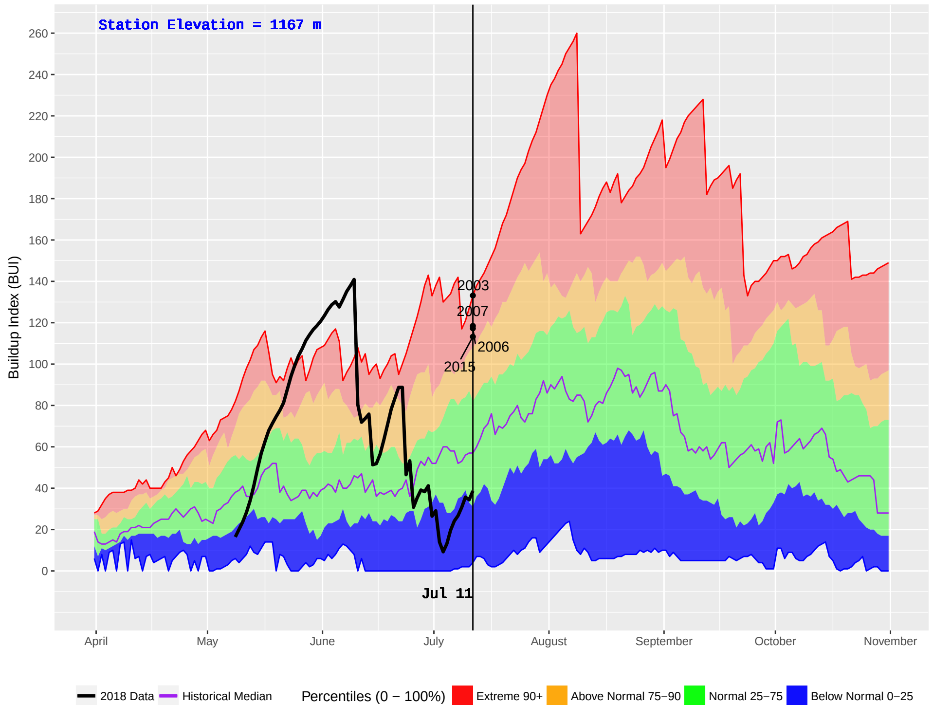
LEIGHTON LAKE (307) : Historical (1982–2016) and Current (2018) Noon Buildup Index (BUI)
